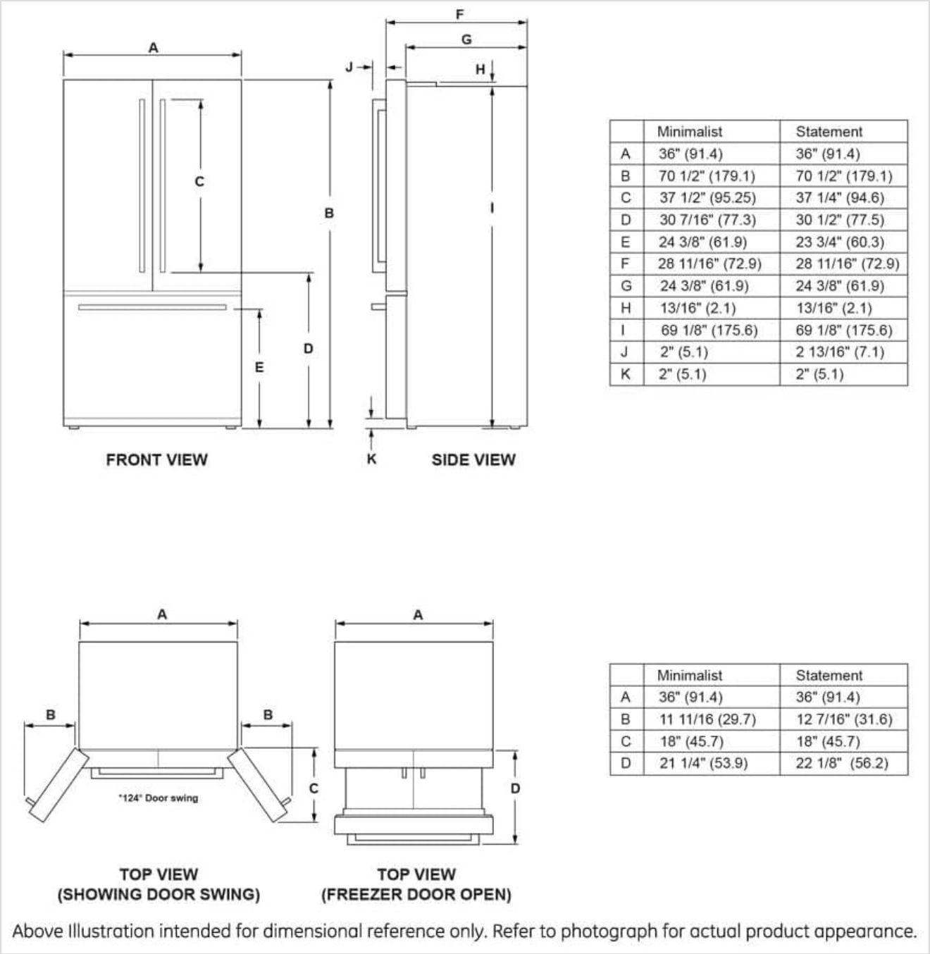
Figure 7.1: Dimensional drawing providing detailed measurements for installation planning. Note that handle dimensions vary by style.
