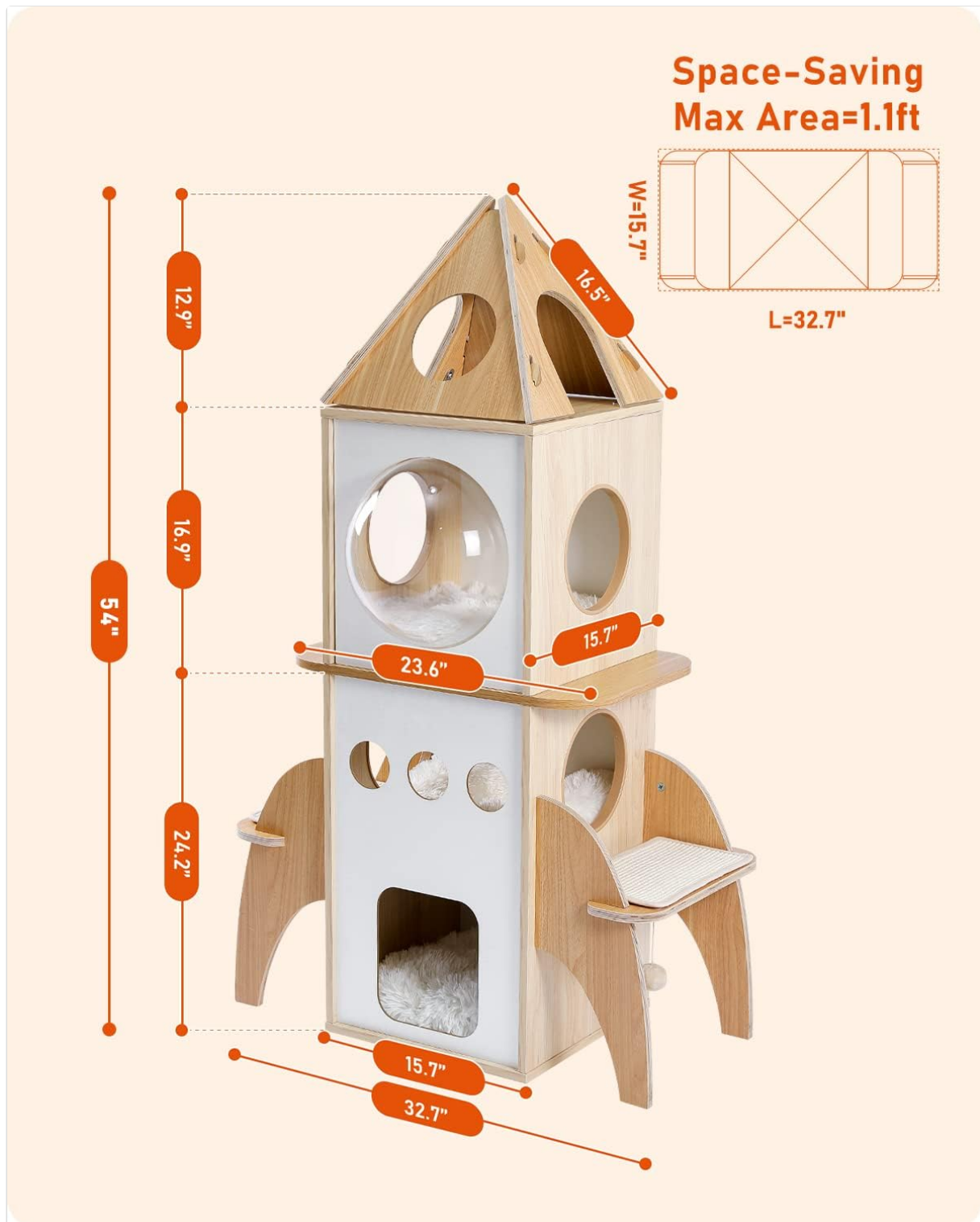
Figure 1: Product dimensions and key components. The cat tree measures approximately 32.7 inches (L) x 15.7 inches (W) x 54 inches (H).
