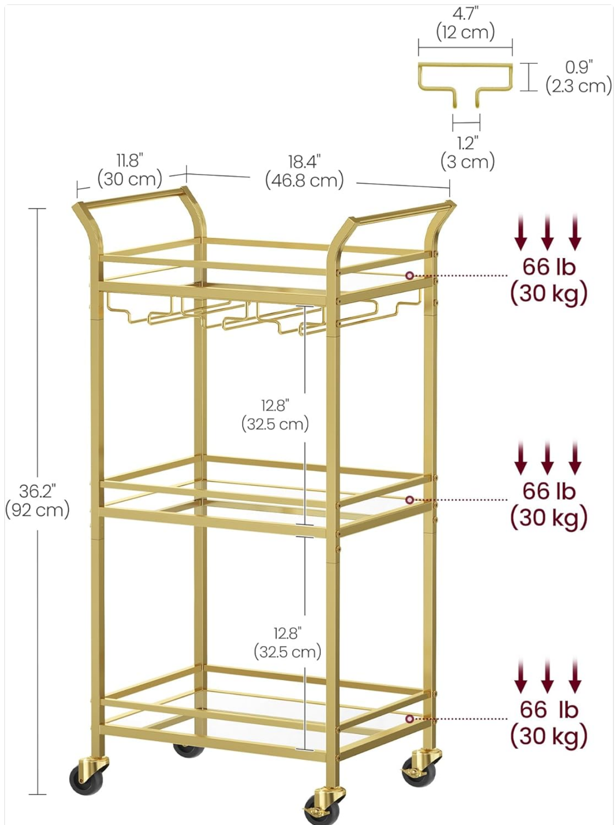
Image 8.1: A technical diagram illustrating the precise dimensions (depth, width, height) and the maximum weight capacity per shelf for the bar cart.
