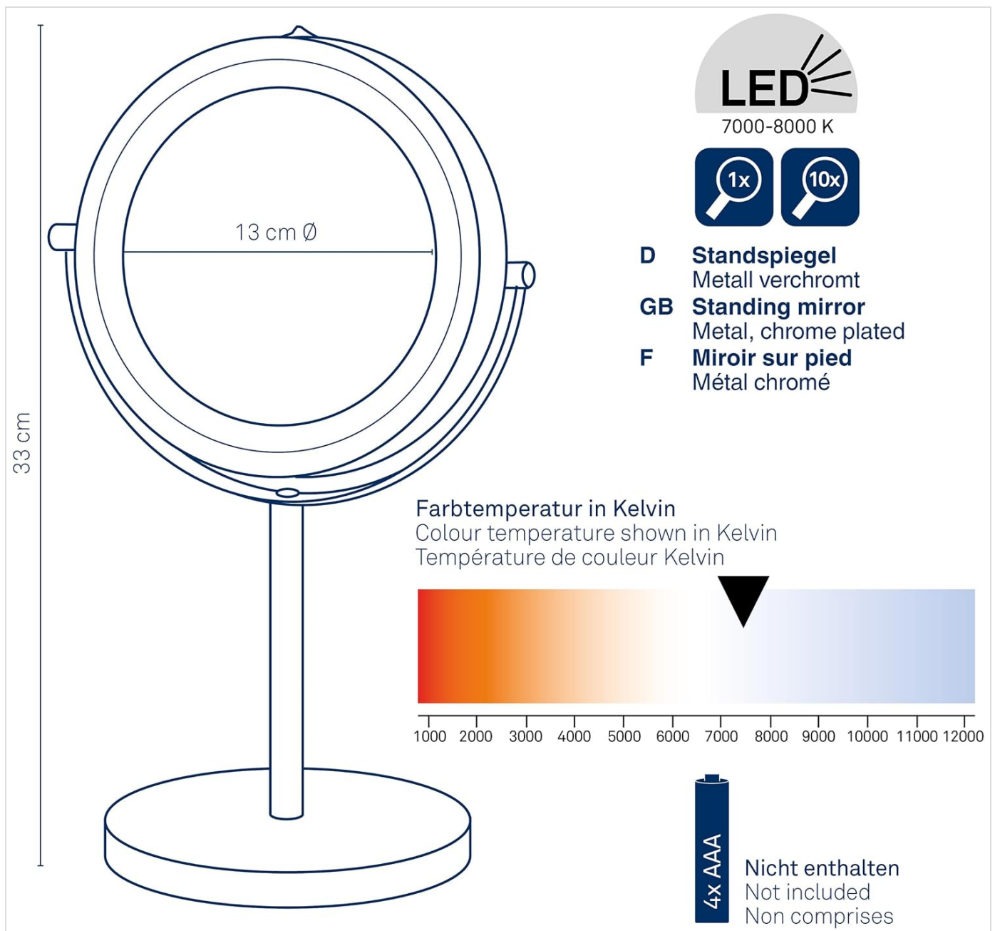
Figure 4: Technical drawing showing dimensions, LED color temperature range, and battery requirements.
