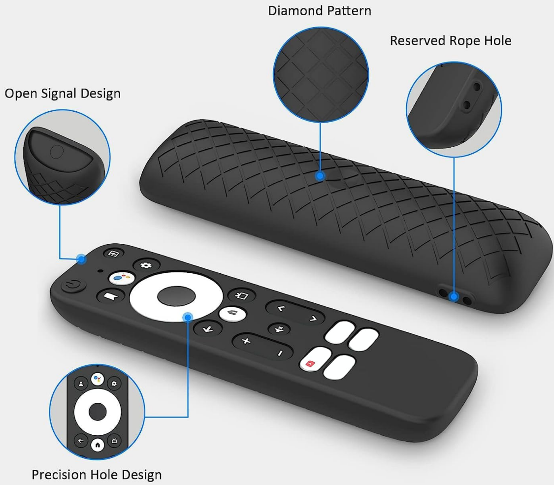
Figure 2: Illustration of the case's precise cutouts for buttons, open signal design, textured grip, and lanyard attachment point.
