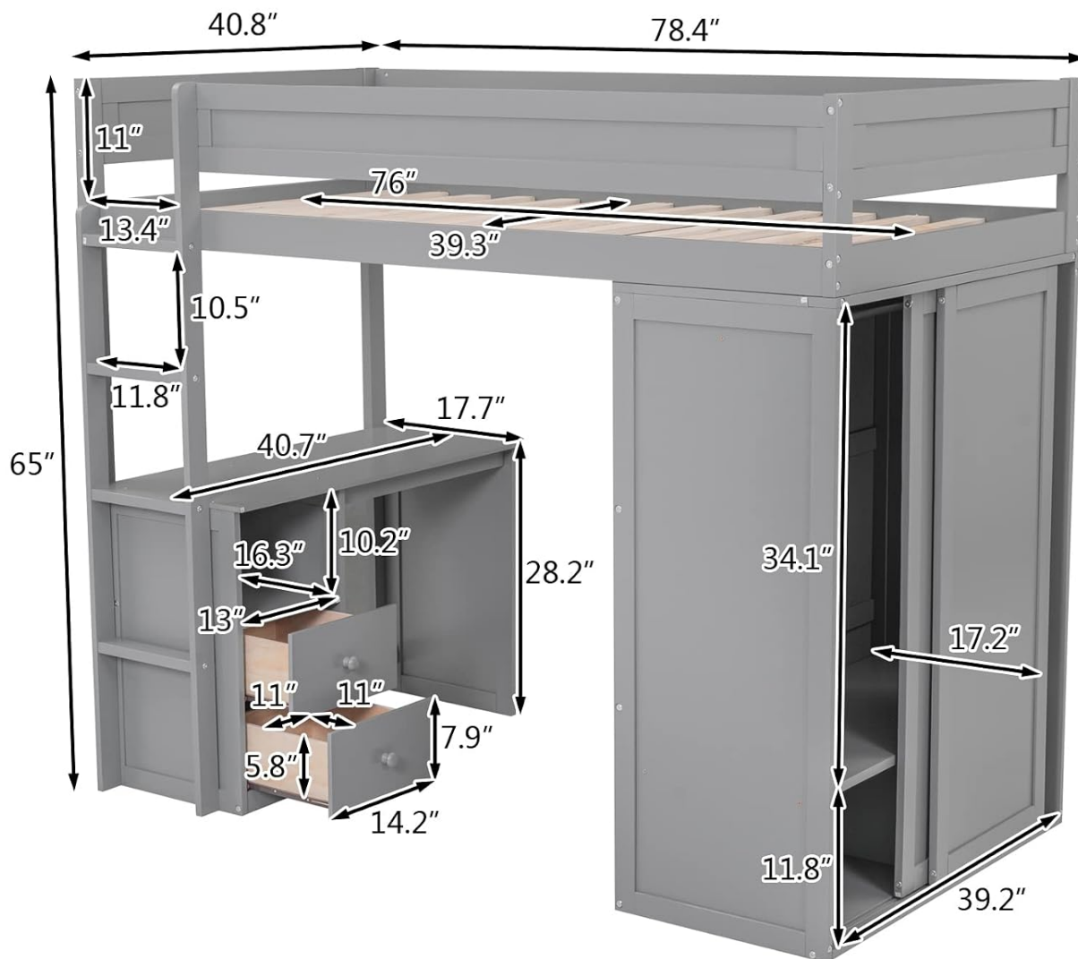
Image 5: Technical diagram illustrating the overall dimensions and key measurements of the VilroCaz Twin Size Loft Bed, including the bed, desk, and wardrobe components.
