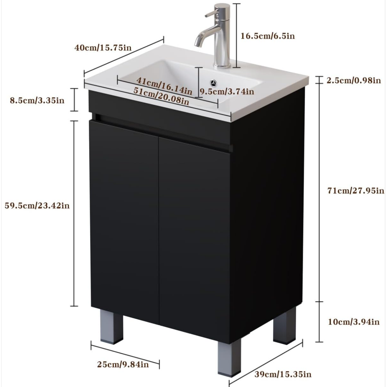
Image 4.1: Detailed dimensions of the vanity and sink for planning.
