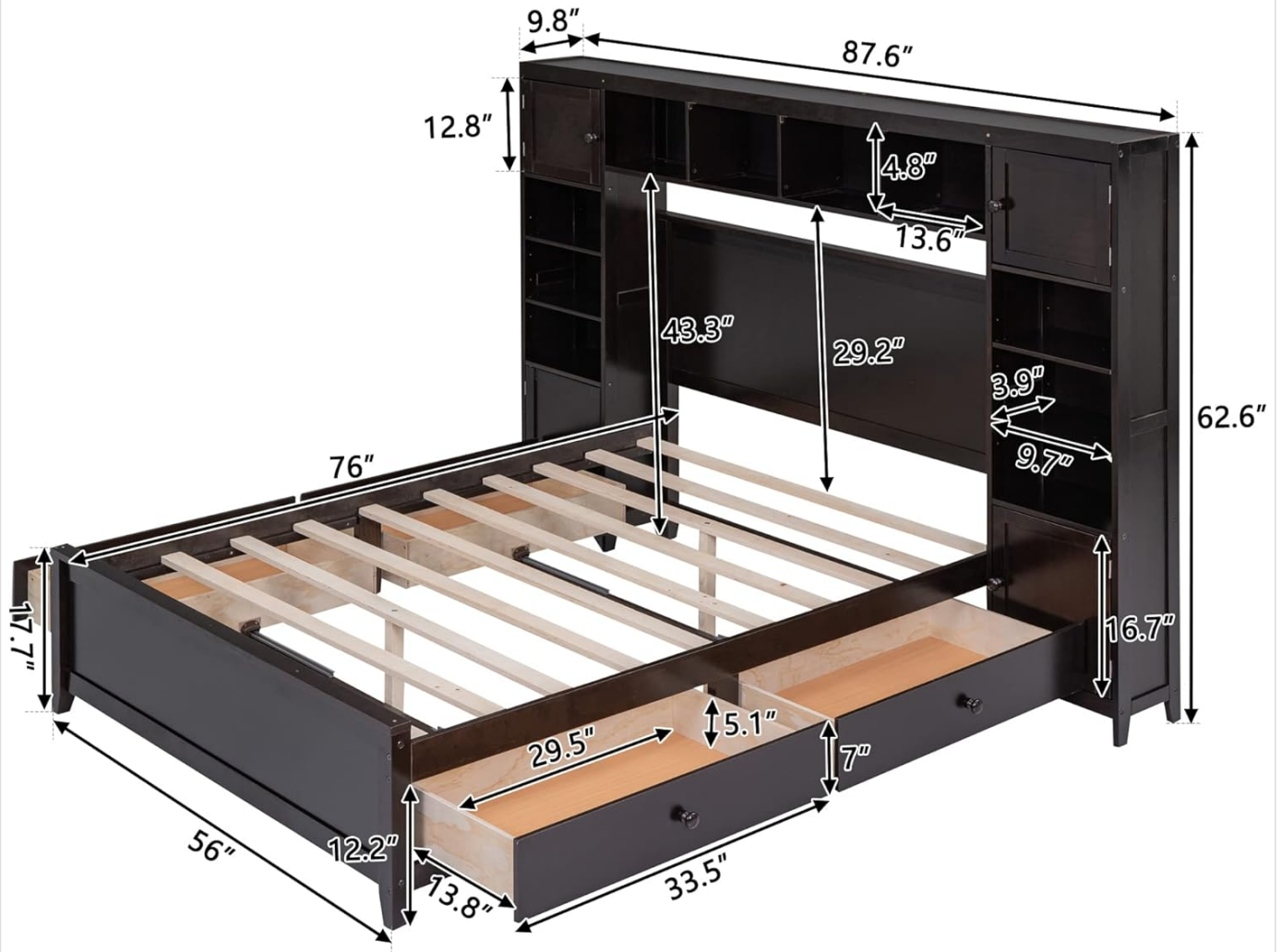
Figure 2: Overall dimensions and key components of the Polibi Full Size Bed Frame.
