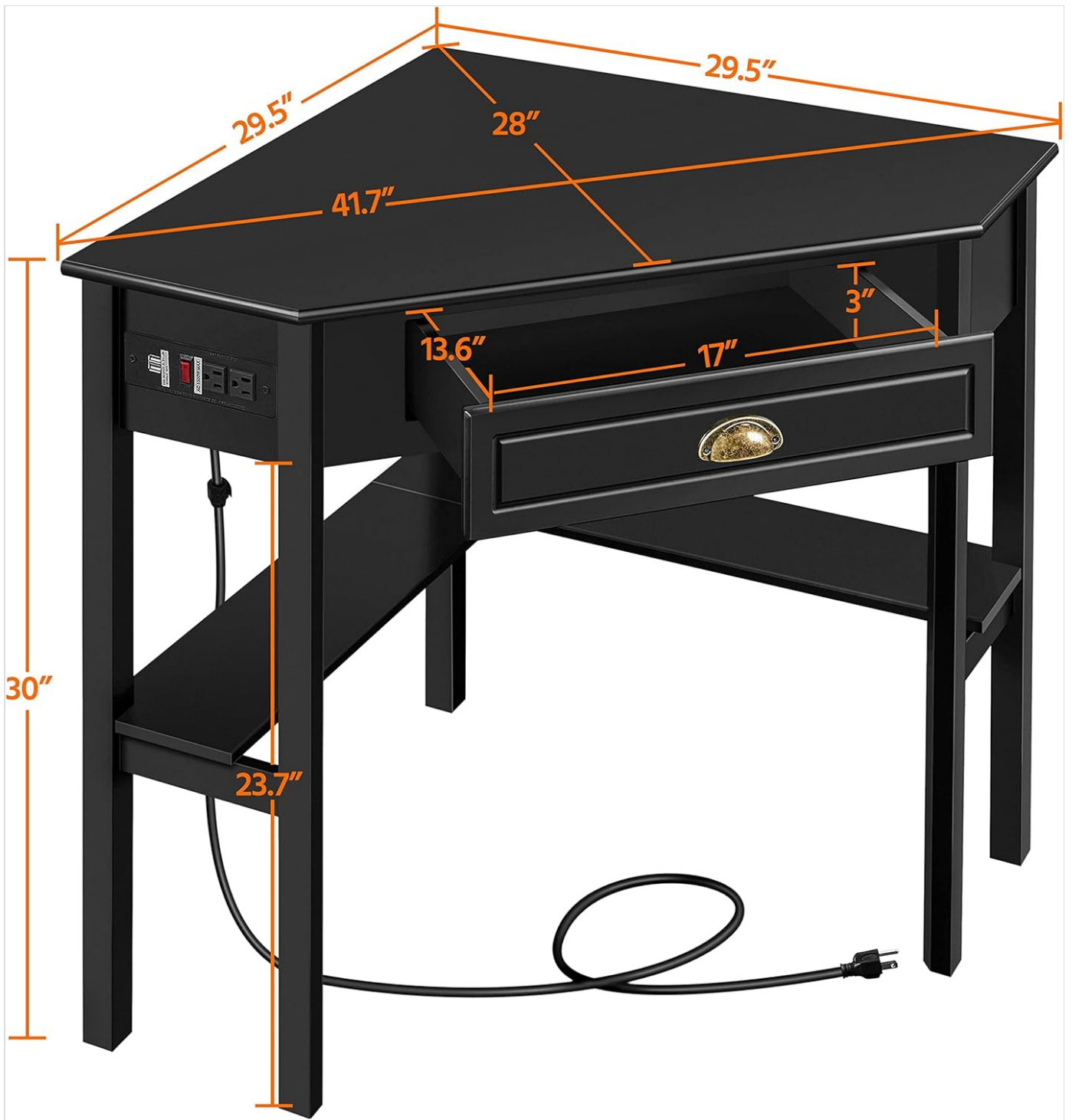
Image: Detailed dimensions of the desk, including desktop width, depth, and height.
