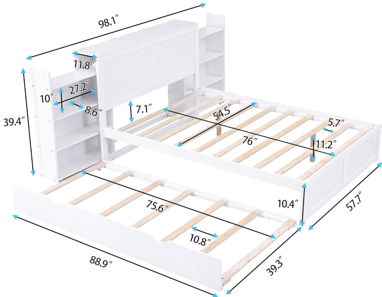
Image 2: Detailed dimensions of the Polibi Full Size Platform Bed and trundle unit.
