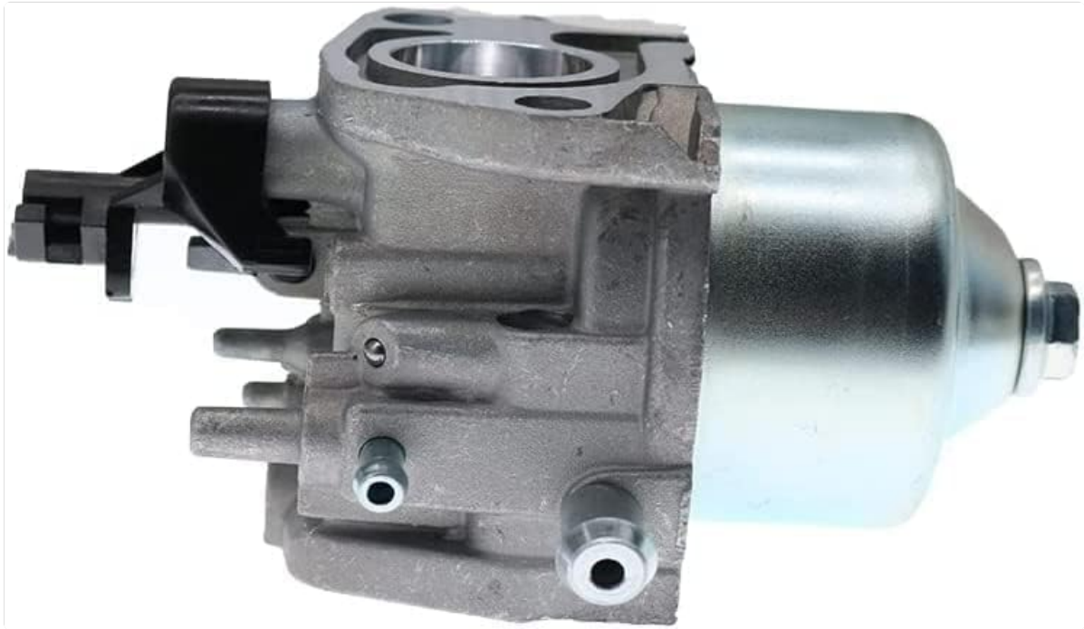
Image: A different side view of the HQParts carburetor, showing additional ports and the float bowl. This view can assist in understanding the internal workings and identifying potential areas for cleaning.
