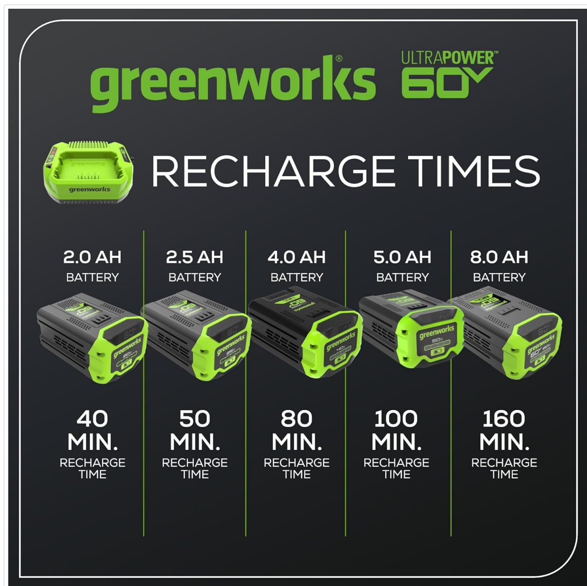
Figure 4: Chart showing approximate recharge times for various Greenworks 60V batteries with the 3A charger.
