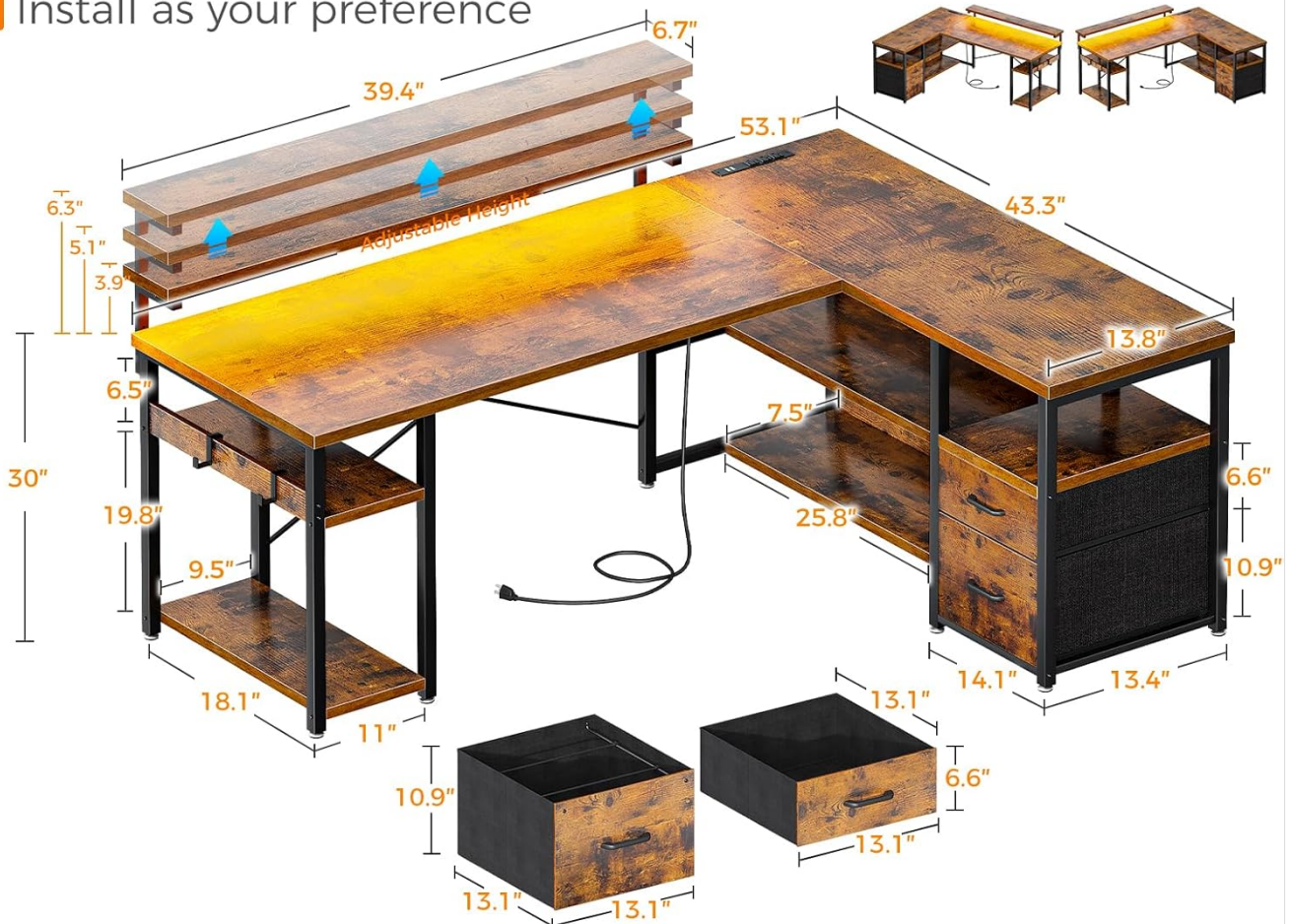
Figure 2: Desk dimensions and reversible assembly options.
