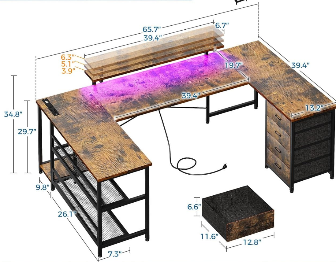
Image: Detailed diagram showing the dimensions of the ODK U Shaped Desk components.
