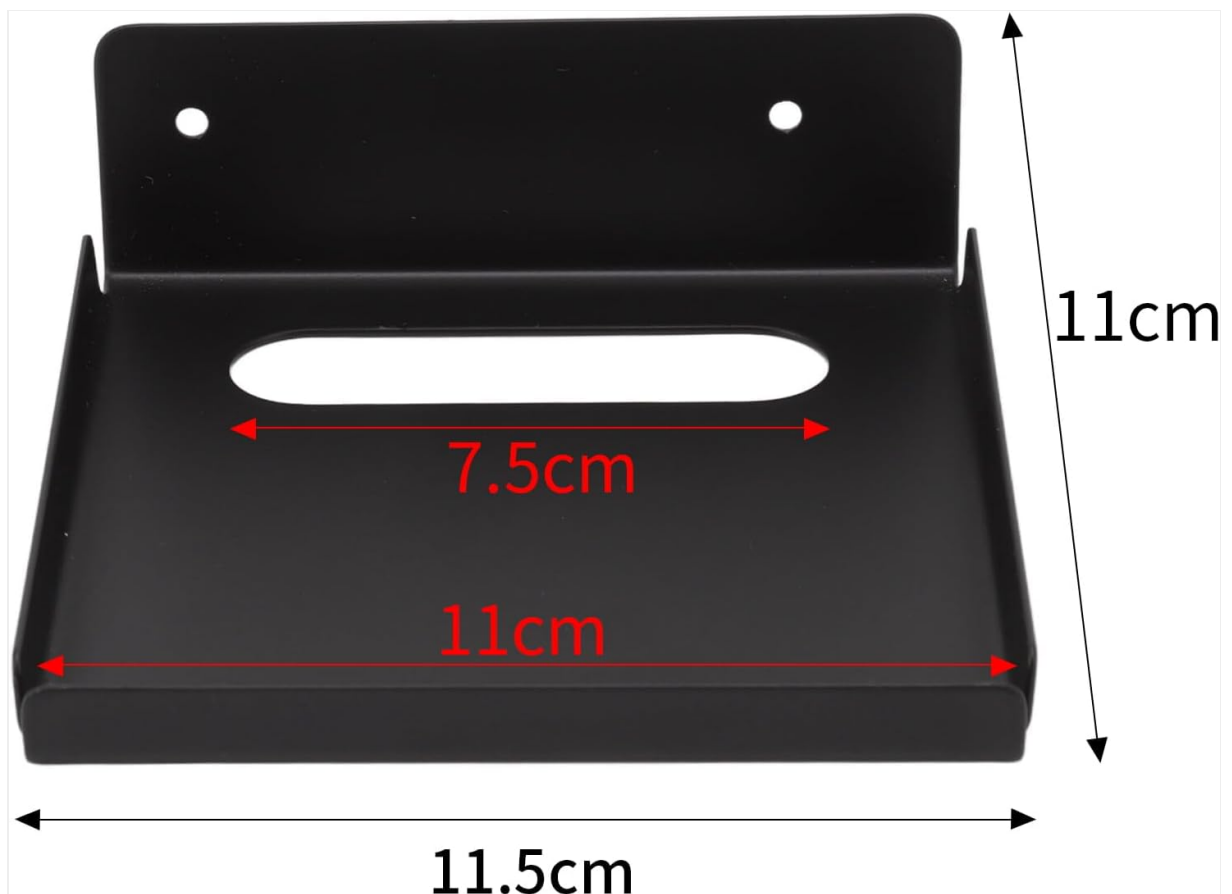
Image: Detailed dimensions of the shelf for planning installation space.
