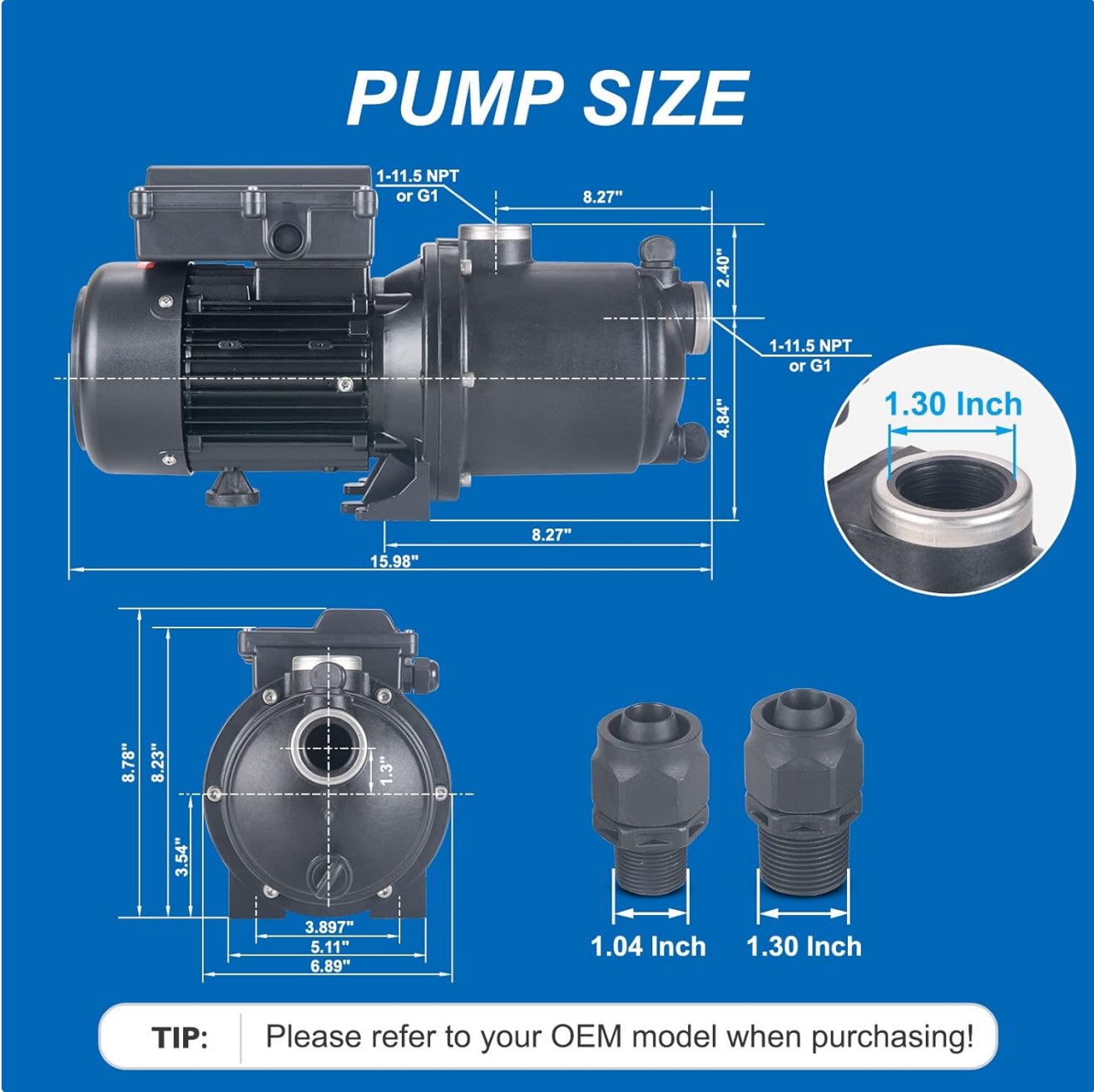
Figure 7.1: Pump dimensions and connection details.
