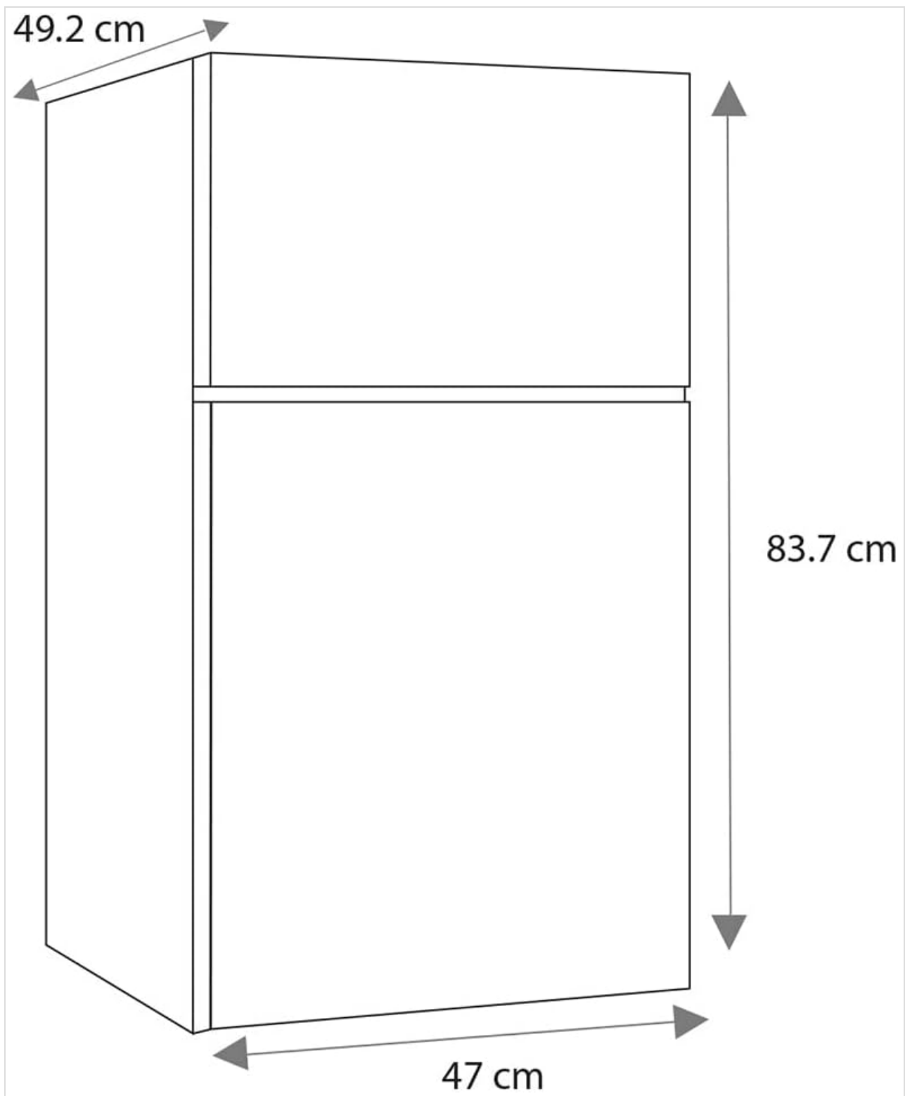
Figure 1: Approximate dimensions of the Mabe RMF032PYMXX mini-refrigerator. Depth: 49.2 cm, Height: 83.7 cm, Width: 47 cm.
