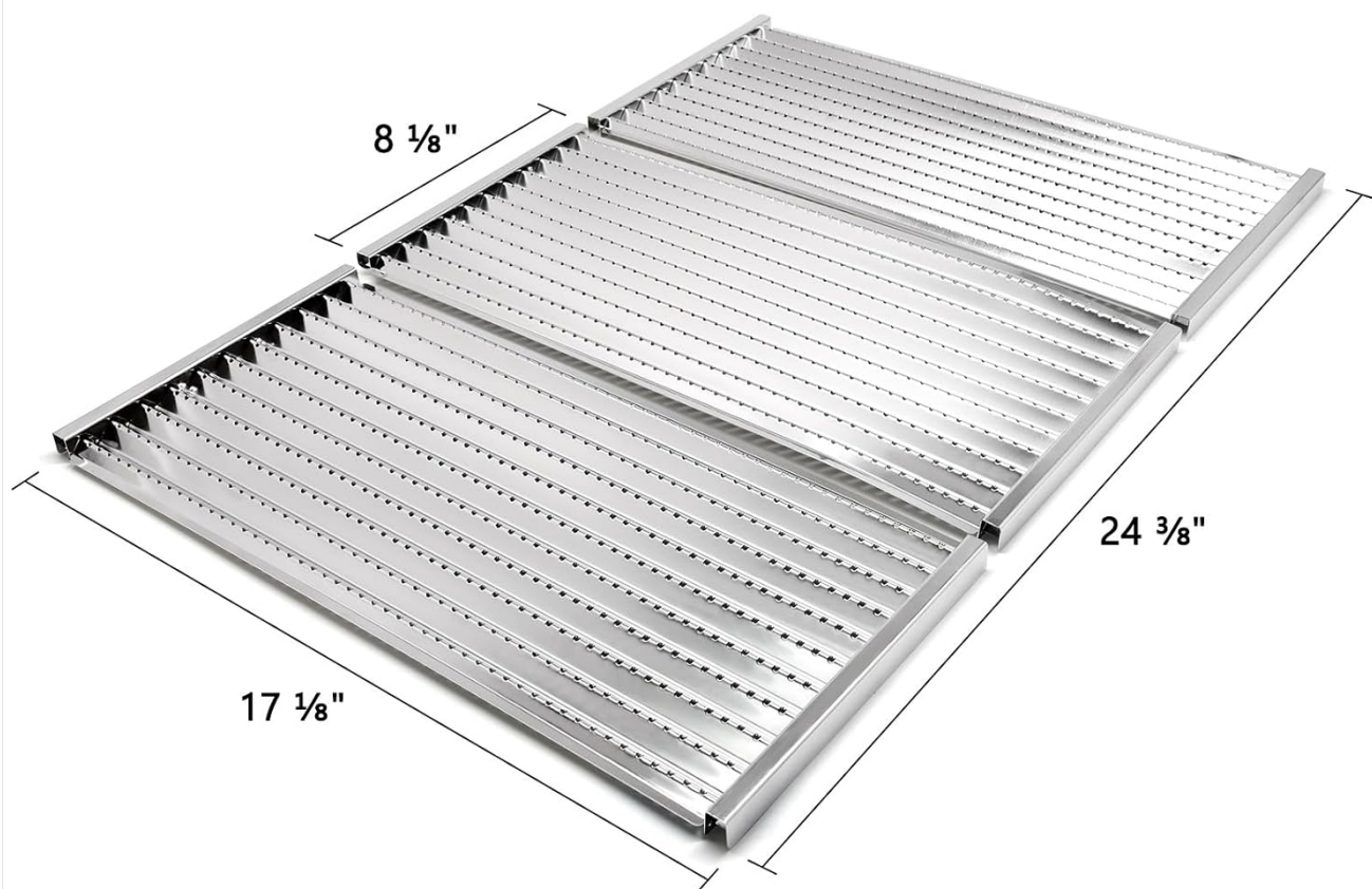
Image: Detailed dimensions of the replacement emitter plates.
