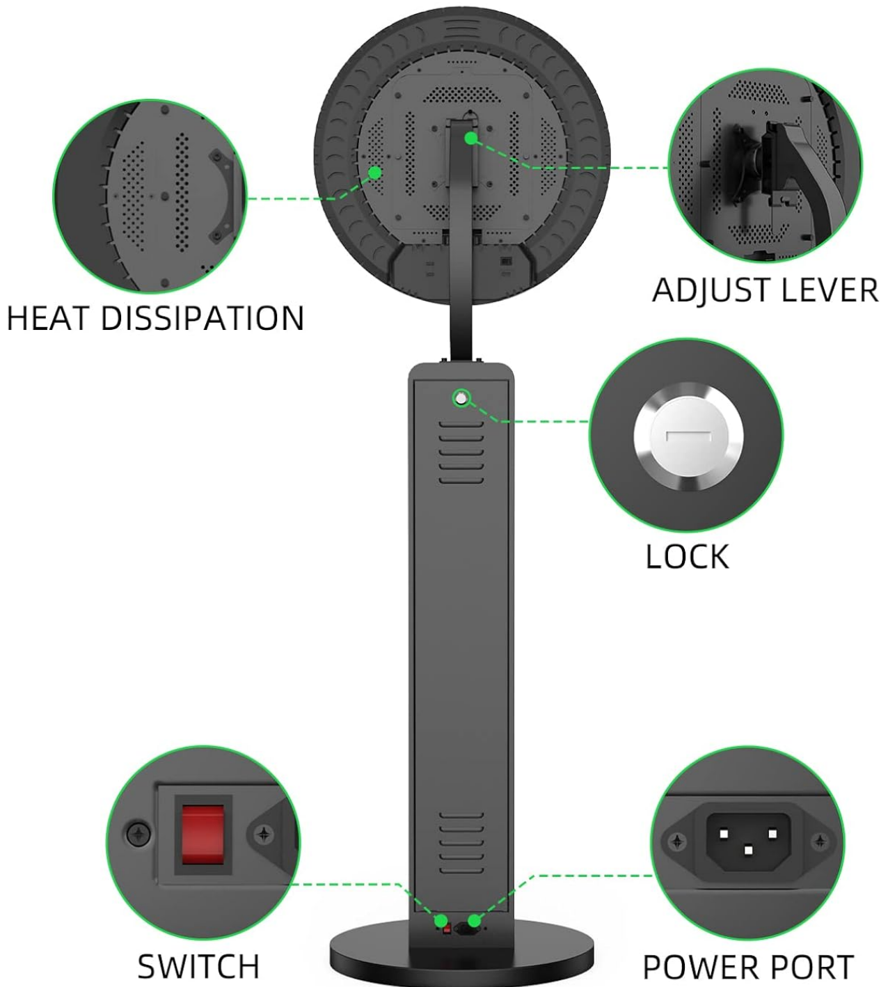
Image 3.2: Key functional areas including the power port, main switch, and adjustment points.
