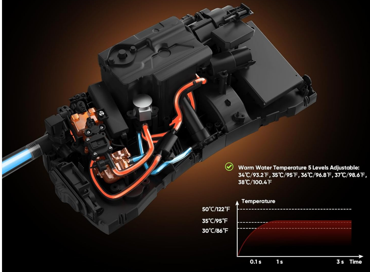
Image: Internal view of the bidet's instant warm water heating system, illustrating the advanced ceramic heating tube that provides and maintains comfortable water temperature.
