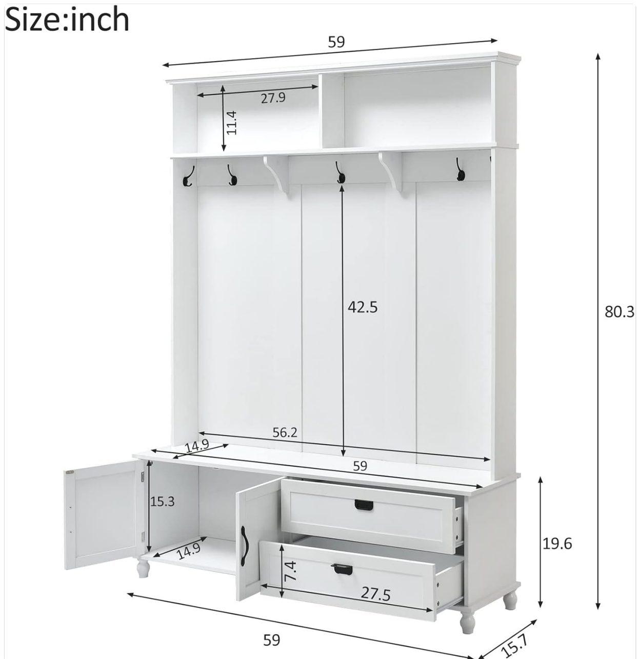
Image: Detailed dimensions of the hall tree.
