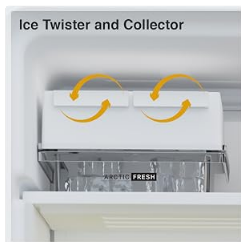
Figure 11: Close-up view of the Ice Twister and Collector in the freezer compartment.
