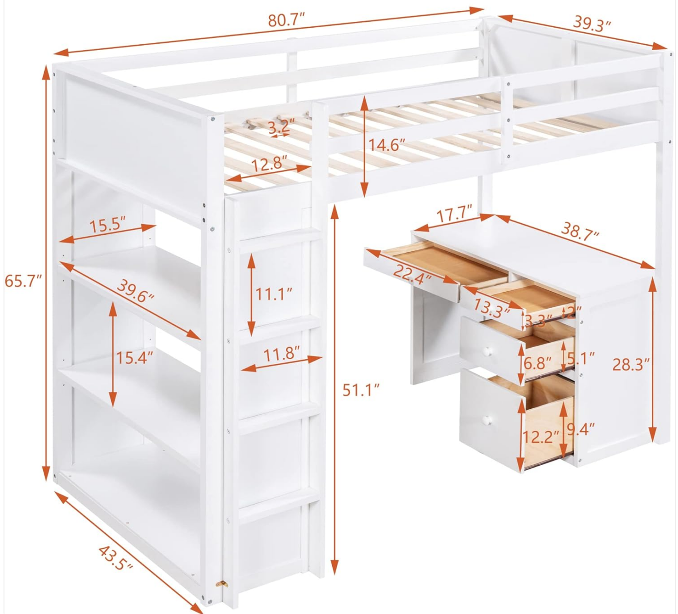
Image: Detailed diagram illustrating the dimensions of the ModernLuxe Twin Size Loft Bed, including overall length, width, height, and specific measurements for the desk, shelves, and ladder steps.
