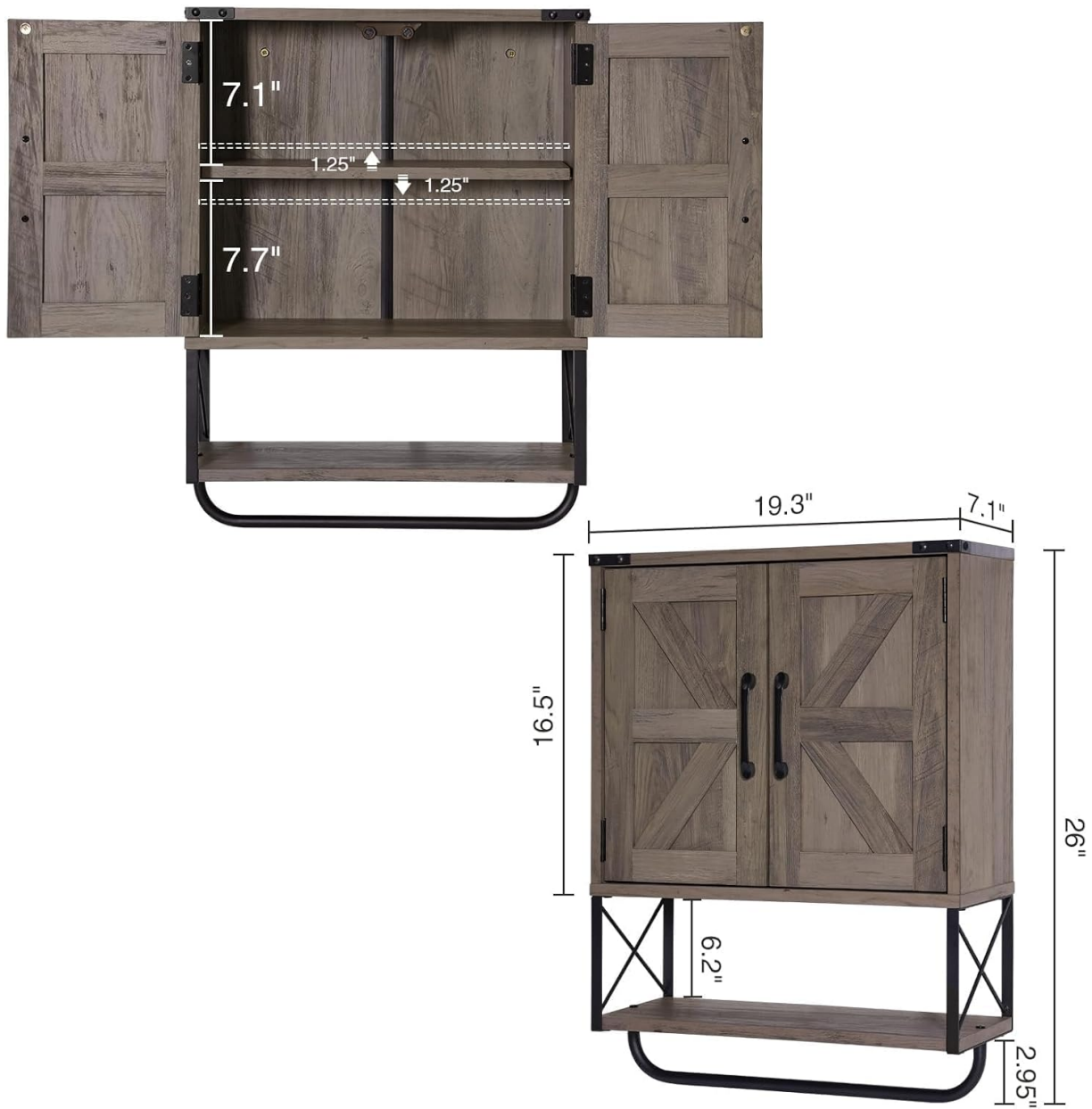
Image: Detailed dimensions of the cabinet, including overall size and interior shelf spacing.
