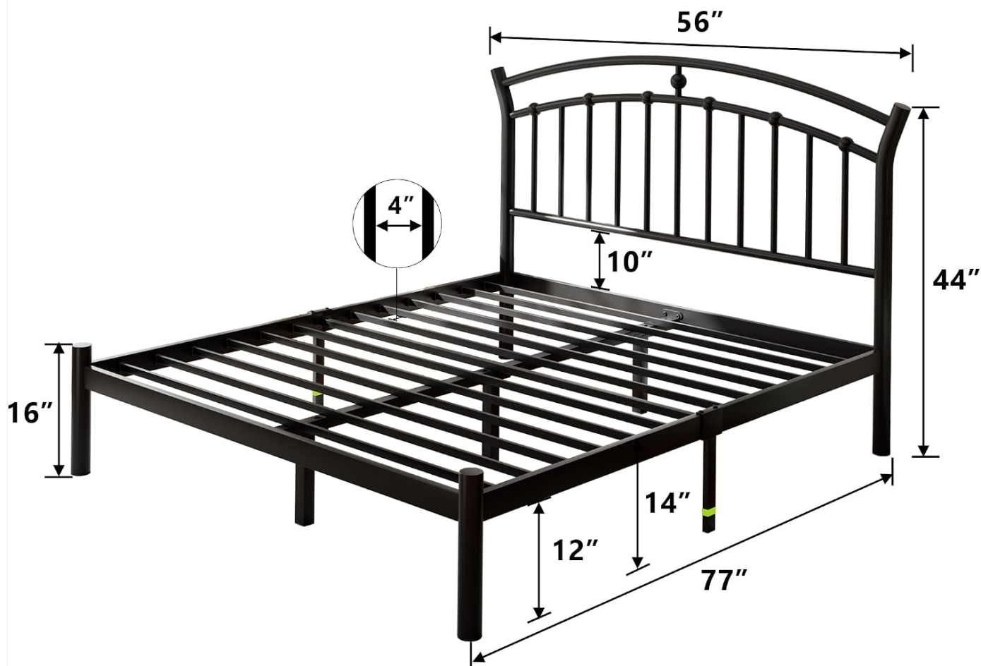
Figure 1: Dimensions of the iPormis Full Size Metal Platform Bed Frame. Overall dimensions are 77"L x 56"W x 44"H, with 12 inches of under-bed clearance and a 1000 lbs weight capacity.
