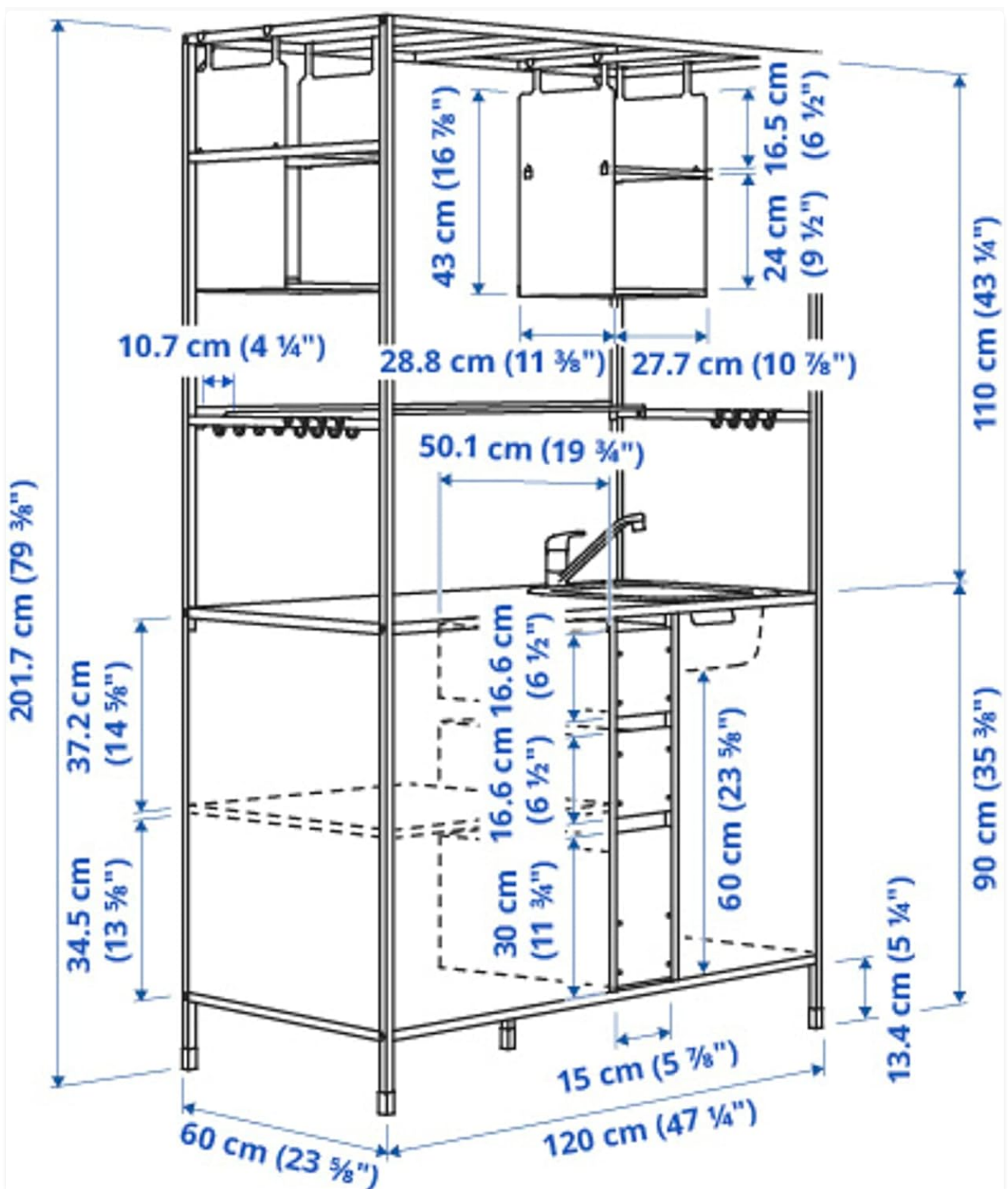
Figure 2: Detailed dimensional diagram of the ÄSPINGE kitchenette, showing overall height (201.7 cm / 79 3/8"), width (120 cm / 47 1/4"), and depth (60 cm / 23 5/8"), along with internal shelf and cabinet measurements.
