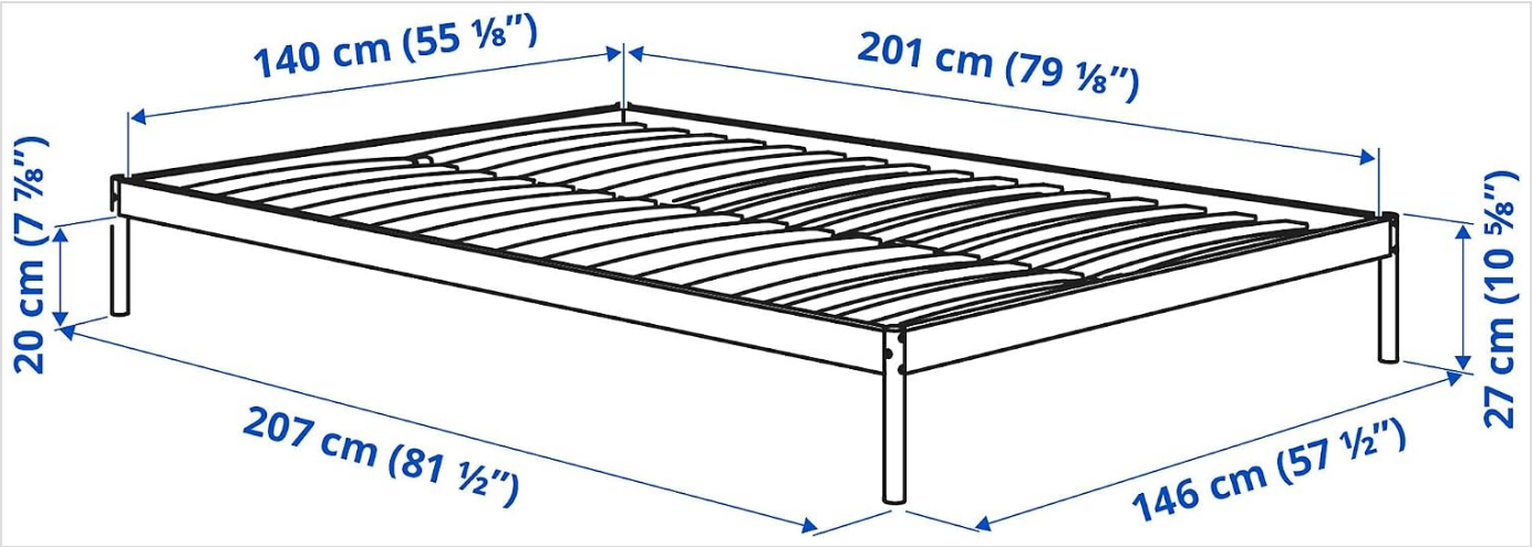
Image 2.1: Detailed dimensional diagram of the VEVELSTAD bed frame, including overall length, width, and height.
