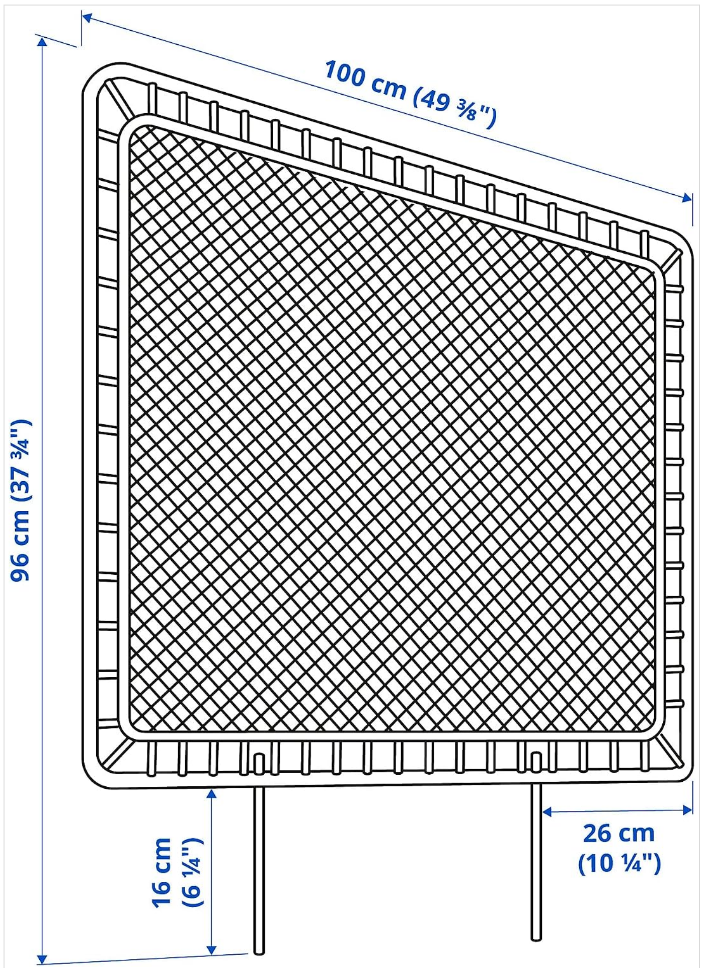
Image 2.2: Detailed dimensional diagram of a single VEVELSTAD headboard, showing its height and width.
