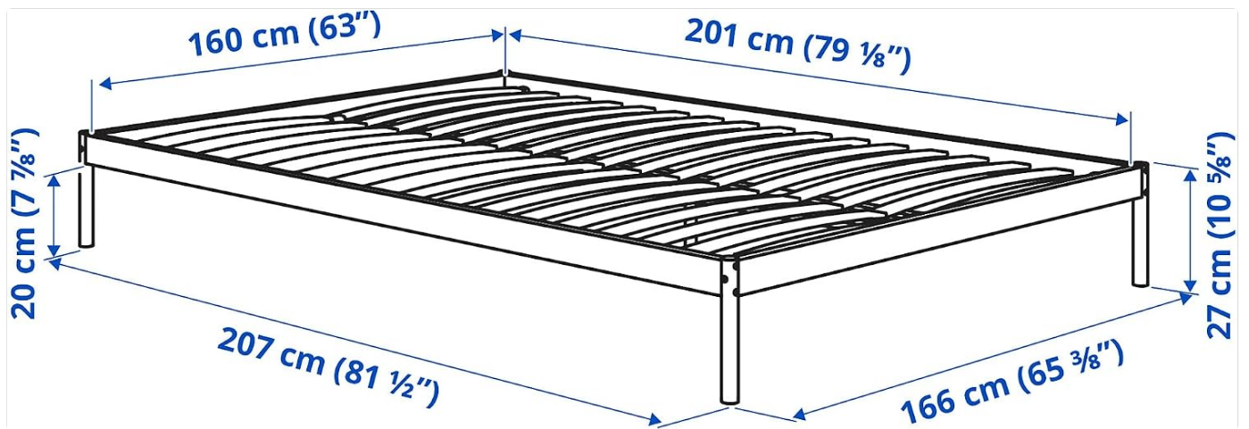
Figure 1: Dimensional diagram of the VEVELSTAD bed frame, showing overall length, width, and height measurements.
