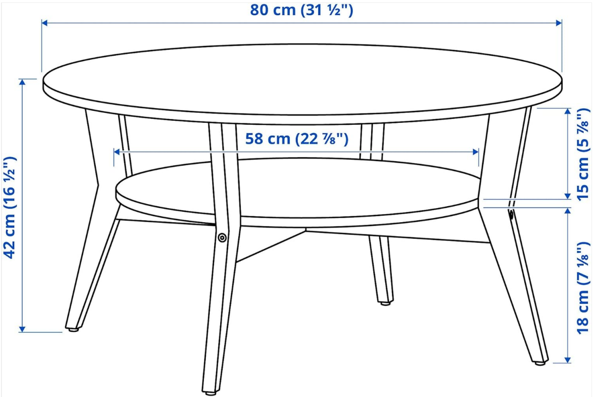
Image 7.1: Dimensional drawing of the coffee table, indicating its overall diameter, height, and lower shelf dimensions.
