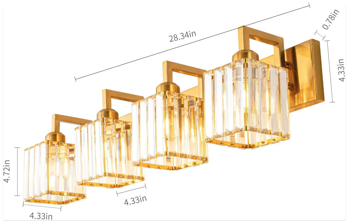
Figure 2: Detailed dimensions of the vanity light, including base length, shade diameter, and projection from the wall.
