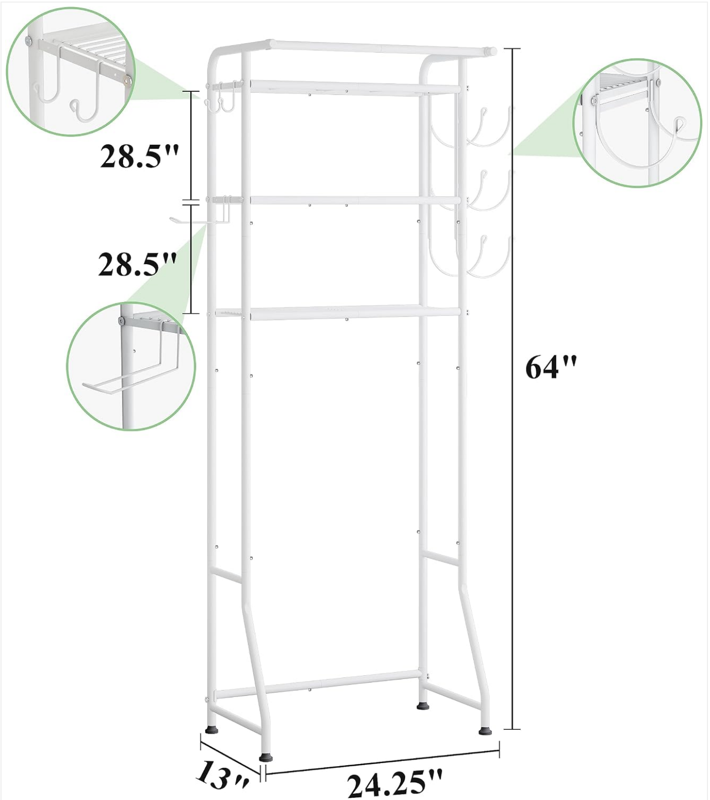
Image: A detailed diagram illustrating the dimensions of the organizer, including width, depth, and height.
