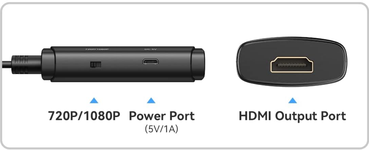
Image 3.1: A detailed view of the converter showing the RCA input port (female), 720P/1080P switch, DC 5V power port, and HDMI output port.
