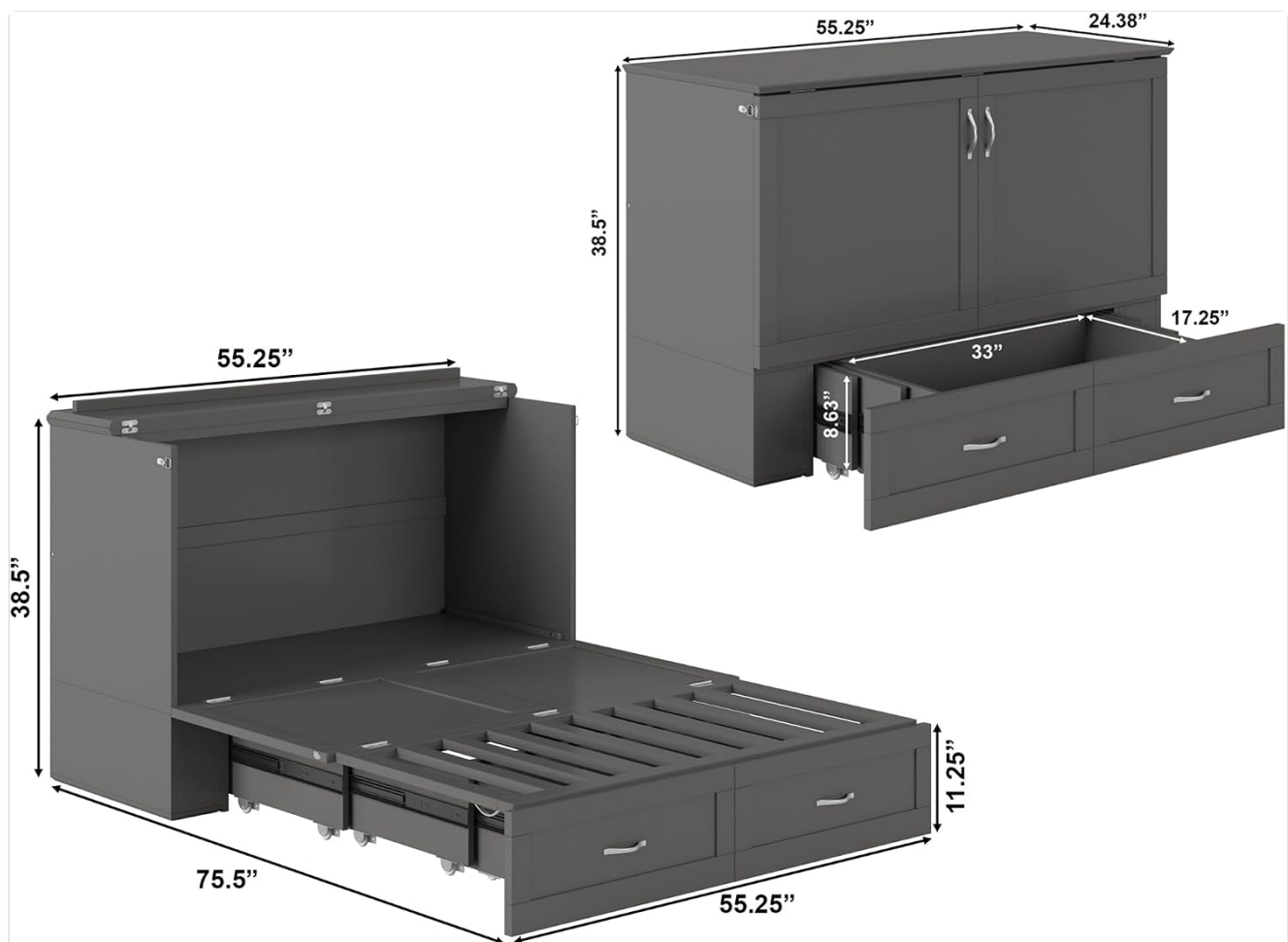
Figure 1: Product Dimensions (Closed: 24.38"L x 55.25"W x 38.5"H; Open: 75.5"L x 55.25"W x 38.5"H)
