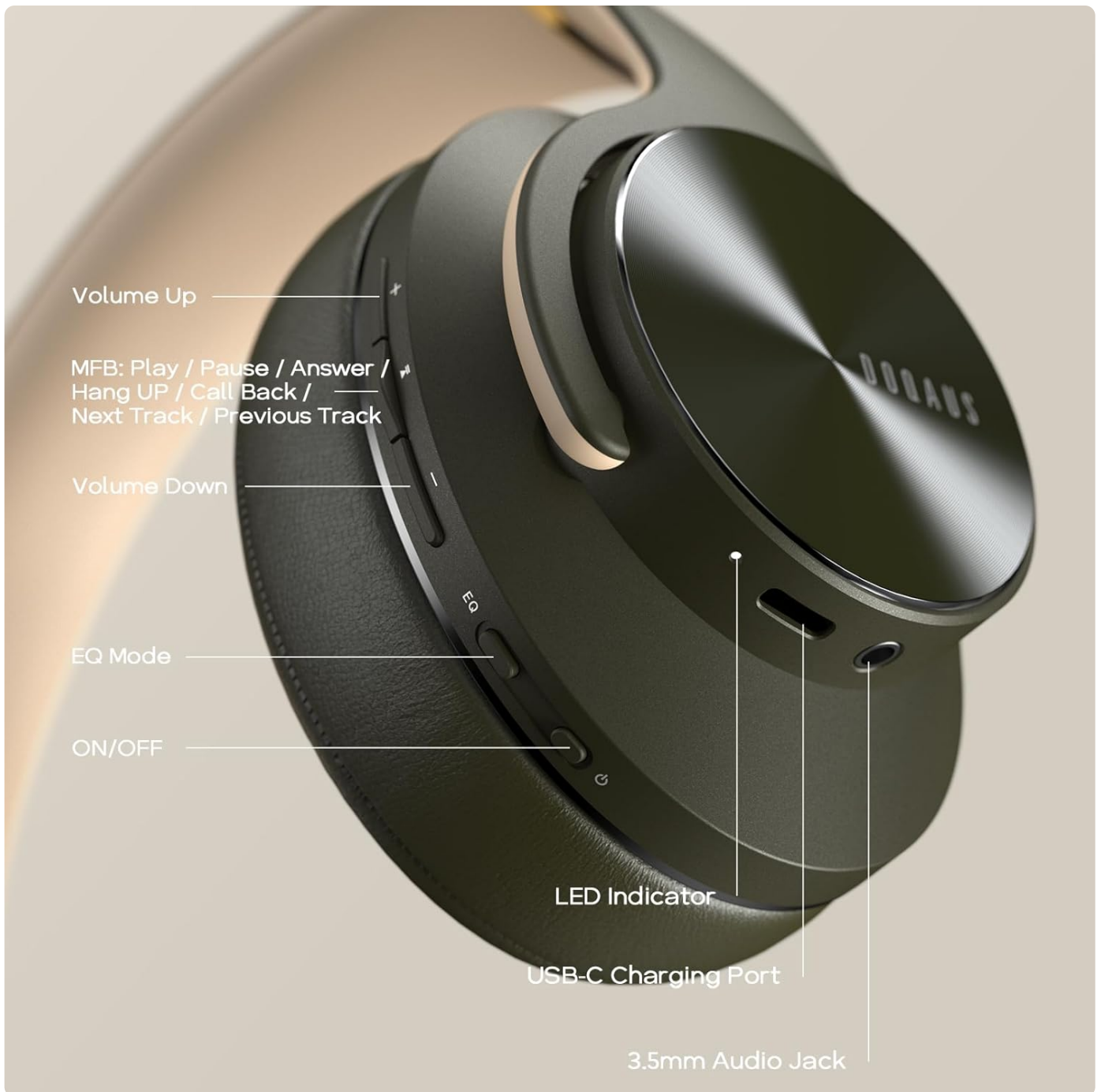
Figure 5: Control layout including Volume Up/Down, MFB, EQ Mode, ON/OFF, LED Indicator, USB-C Charging Port, and 3.5mm Audio Jack.
