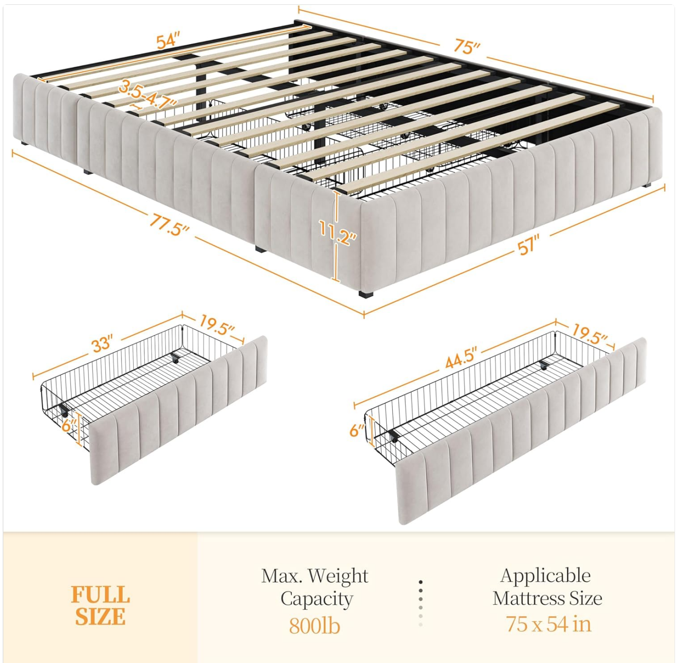
Figure 5: Diagram illustrating the dimensions of the Yaheetech Full Bed Frame, including overall length, width, height, and drawer sizes.
