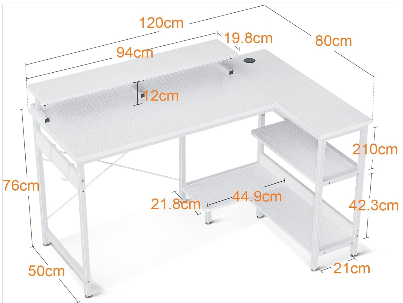
Image: A detailed diagram illustrating the dimensions of the ODK L-Shaped Corner Desk, providing measurements for the main desktop, side shelves, monitor stand, and overall height.
