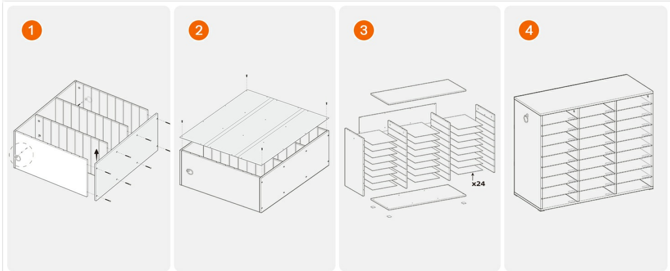
Figure 1: Exploded view of all components and hardware.
