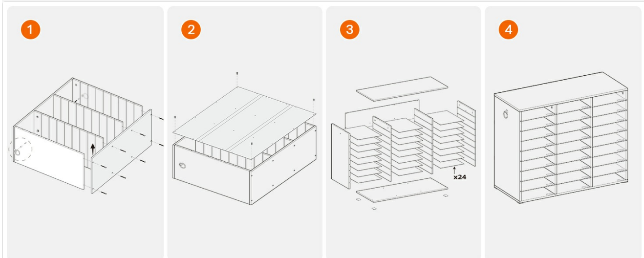
Figure 2: Visual guide for assembly steps.
