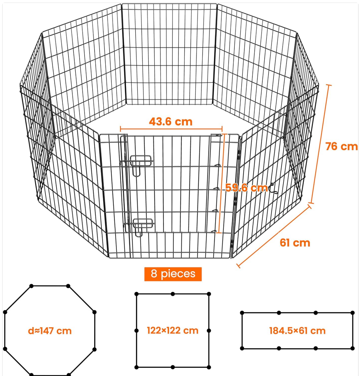
Figure 3.1: Package contents and dimensions. The diagram illustrates the 8 panels, connecting rods, and the overall dimensions of the playpen when assembled in an octagonal shape, with each panel measuring approximately 61 cm wide and 76 cm high.
