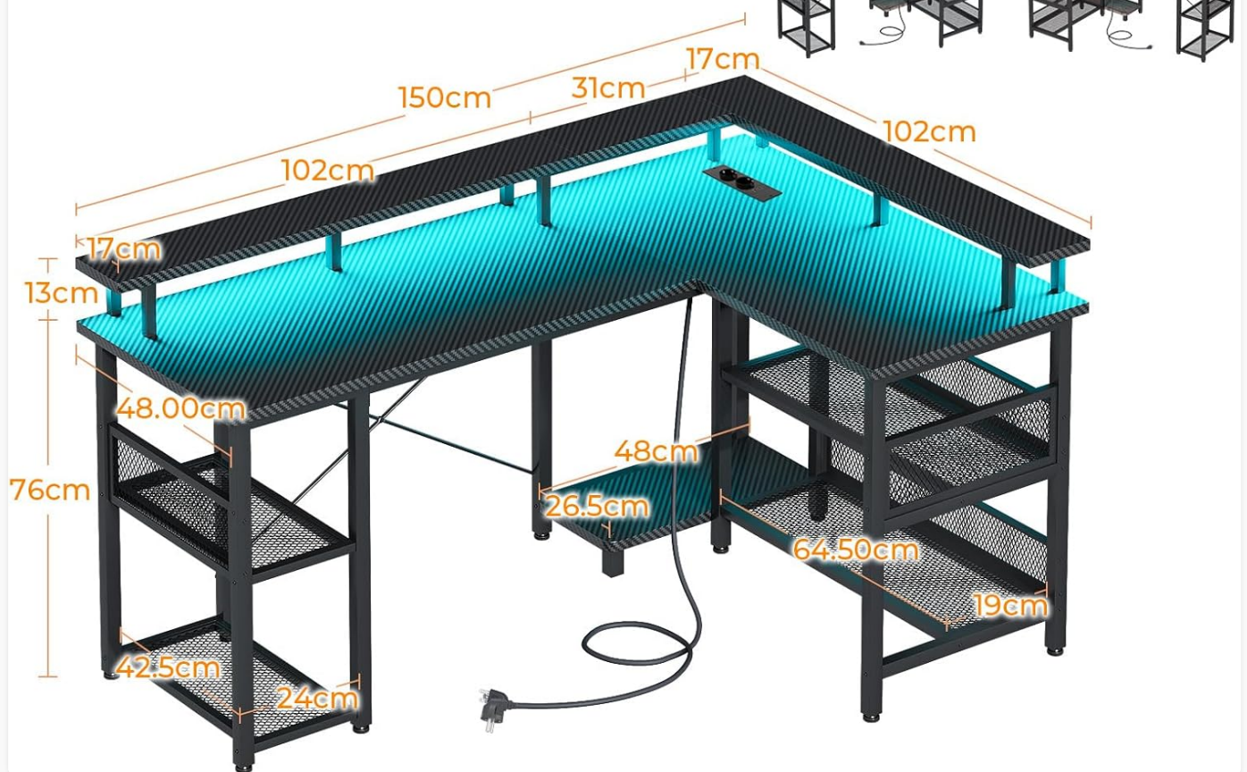
Figure 2.2: Illustration of the desk's reversible design and overall dimensions (150cm x 102cm x 88.7cm).
