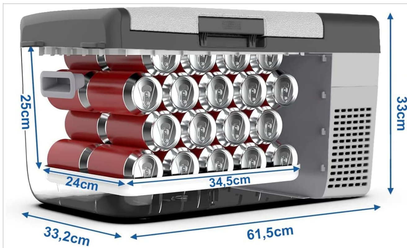
Image 3.1: Detailed dimensions of the ICECO MCD20S, showing its length (61.5 cm), width (33.2 cm), and height (33 cm).
