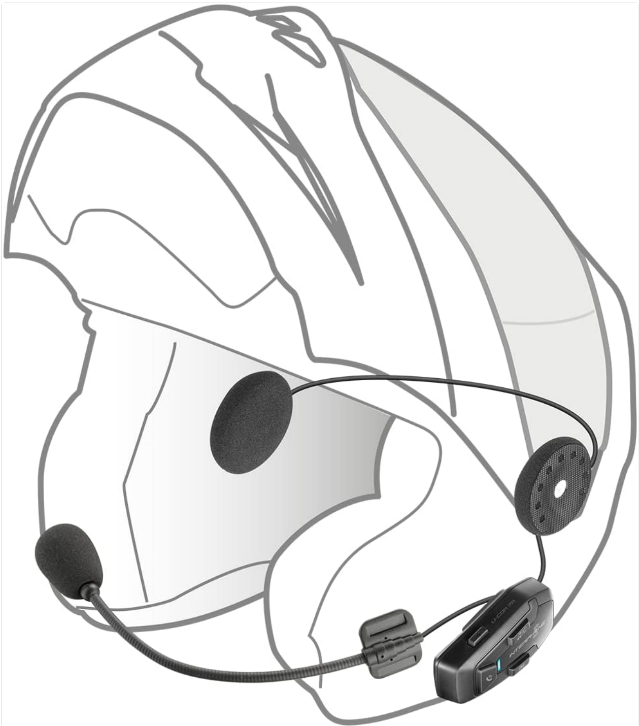
Image: Installation diagram for the UCOM7 with boom microphone in an open-face helmet.
