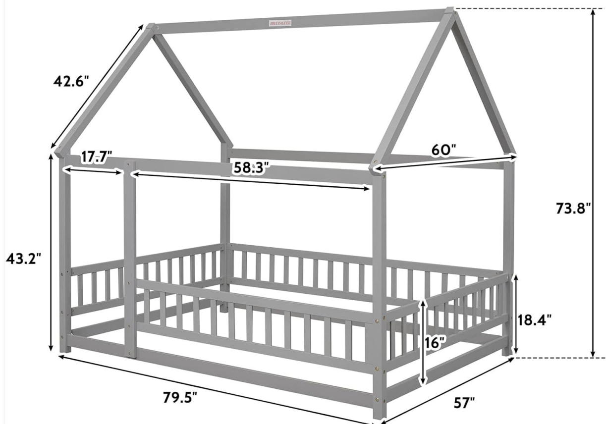
Image 4.1: Detailed dimensions of the LLS Full Size Floor Bed Frame, including length, width, and height measurements.
