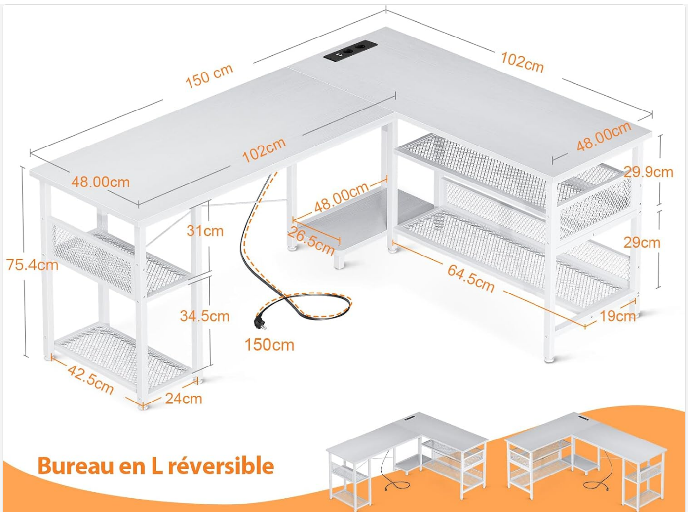
Figure 3: A detailed diagram showing the dimensions of the ODK L-shaped desk, including the main desktop, side shelves, and power cord length.
