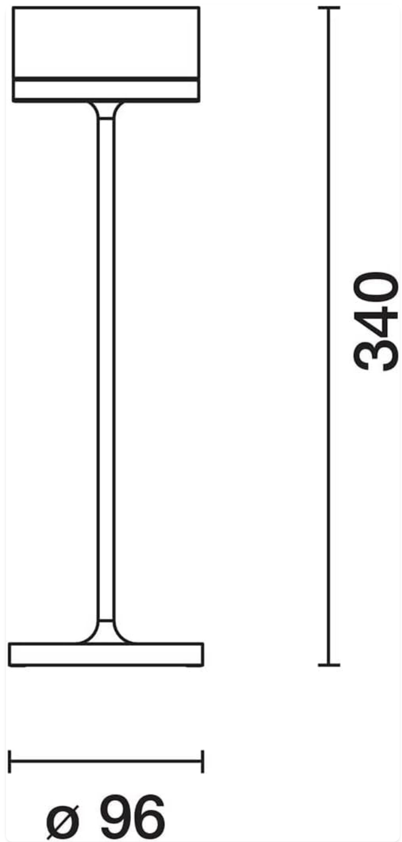
Figure 4: Lamp Dimensions Diagram
