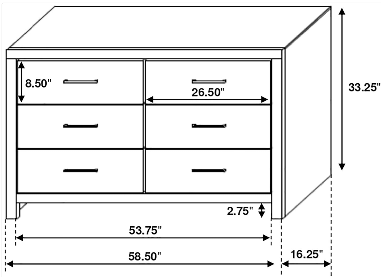
Image: Diagram illustrating the dimensions of the Dresser, including width, depth, and height measurements.
