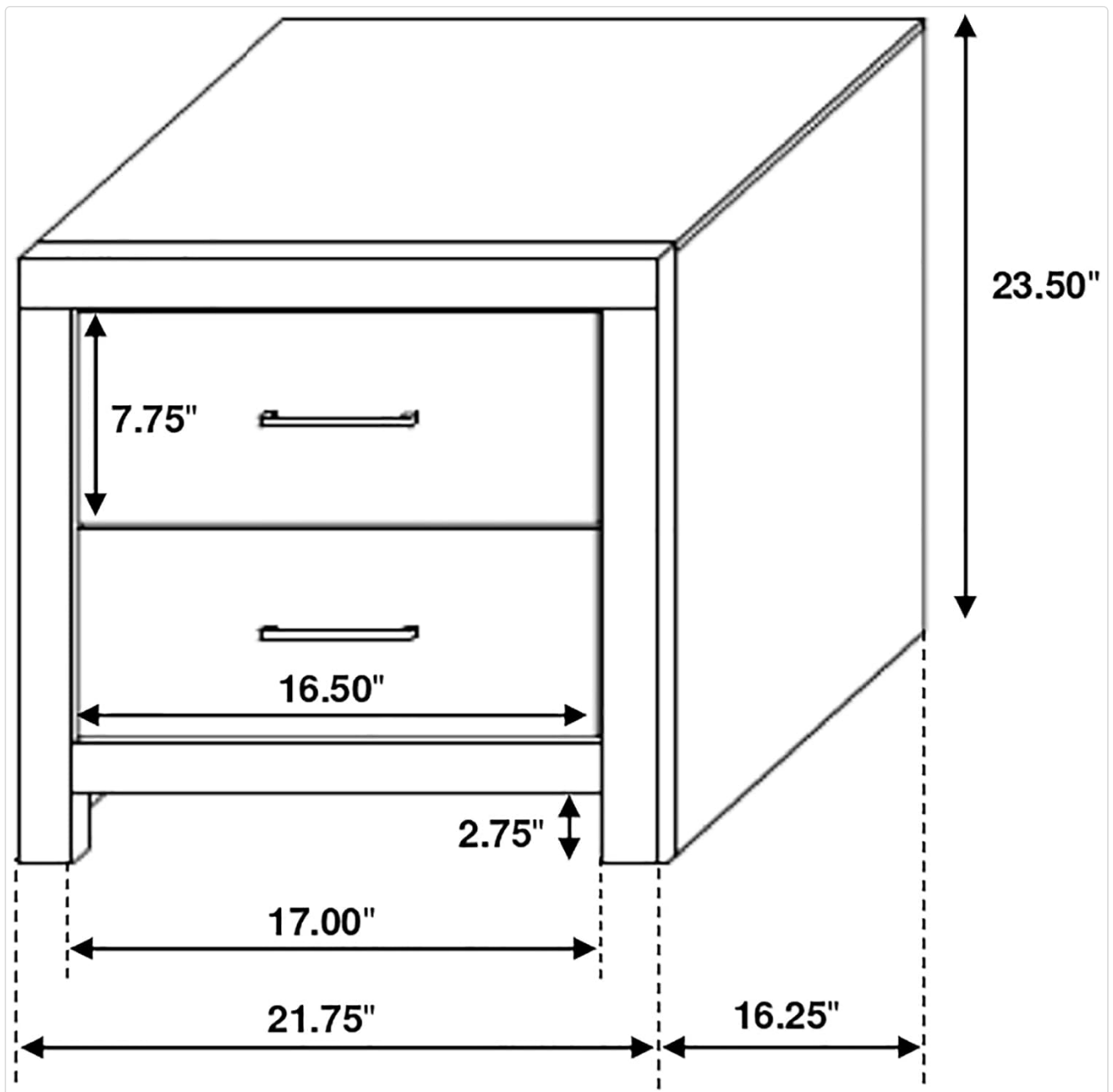
Image: Diagram illustrating the dimensions of the Nightstand, including width, depth, and height measurements.
