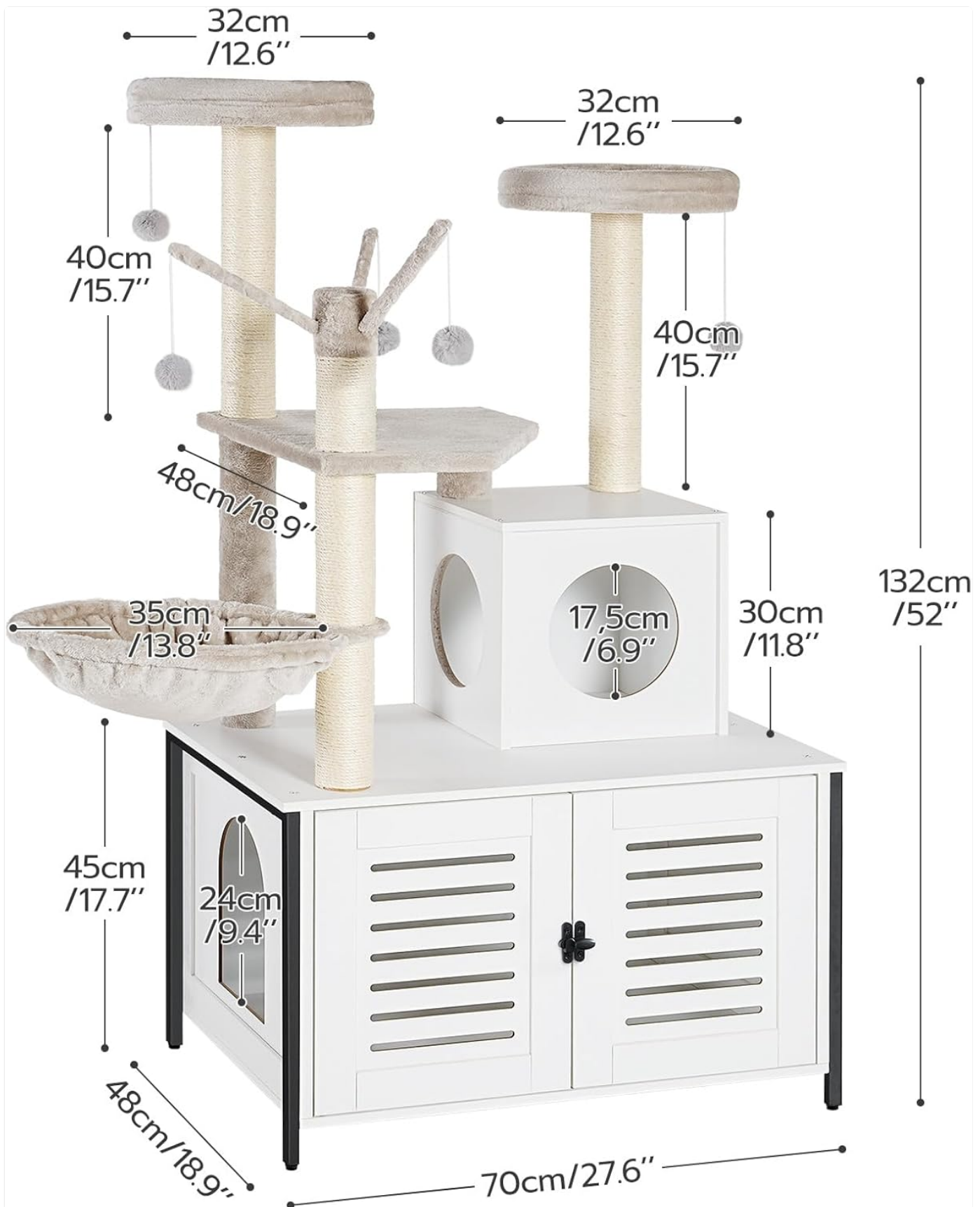
Image: Comprehensive dimension diagram of the cat tree, indicating various measurements in both centimeters and inches.
