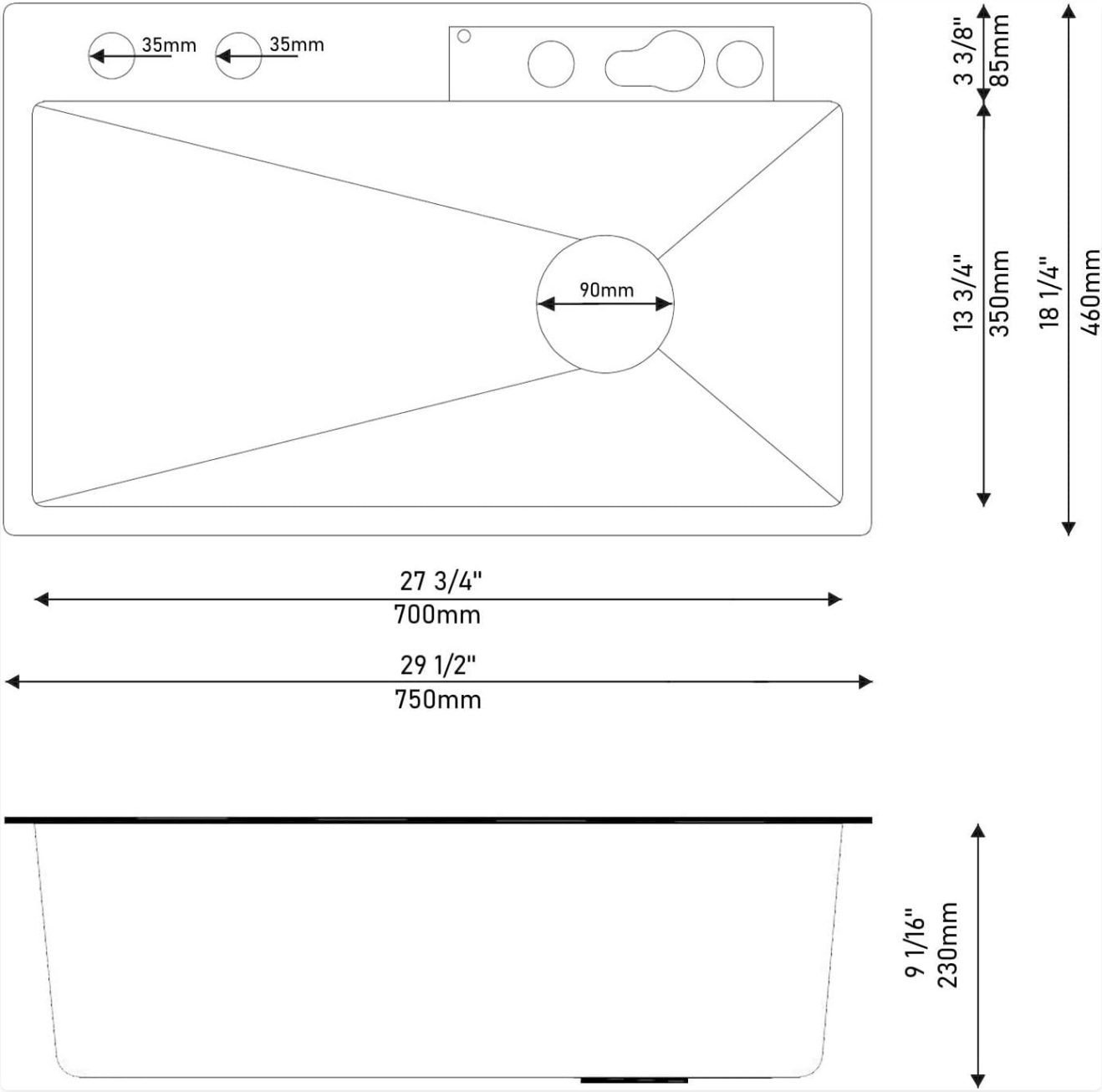
Figure 7.1: Product Dimensions Diagram
