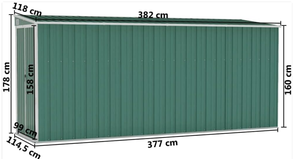
Image: Dimensional diagram of the garden shed, indicating overall measurements.
