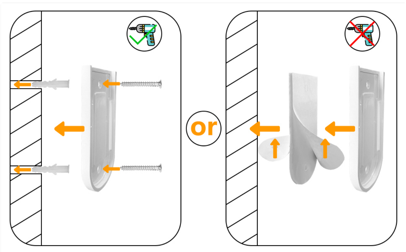
Image: A diagram illustrating the two optional installation methods for the lamp: using adhesive tape for flat surfaces or screws and wall anchors for uneven surfaces.
