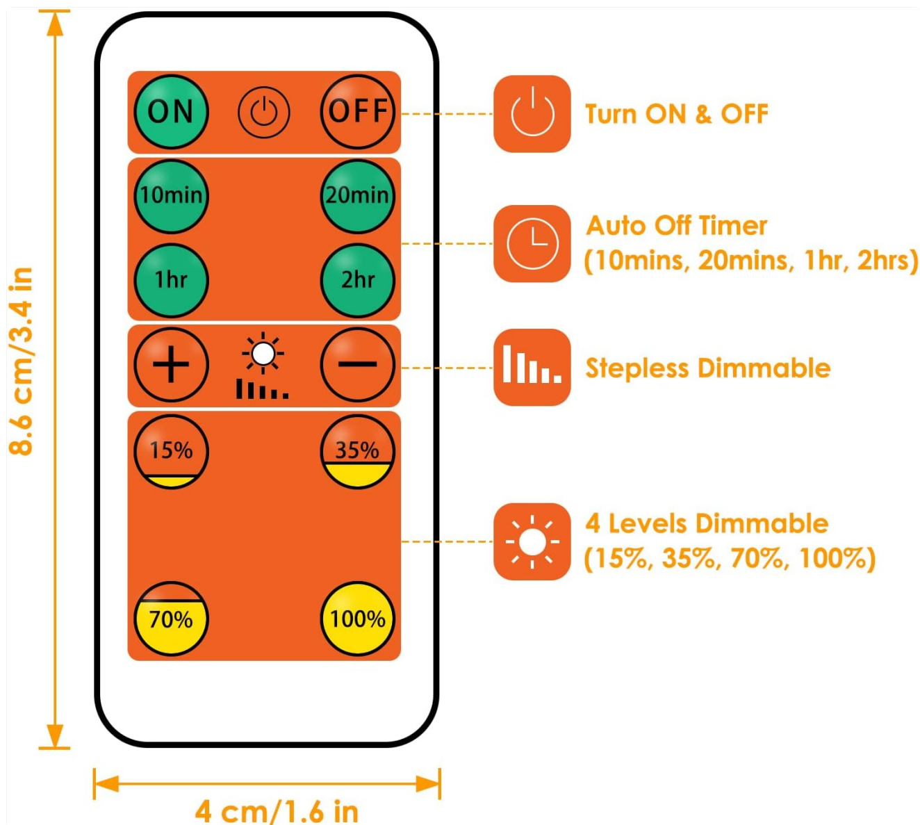
Image: A detailed diagram of the wireless remote control, highlighting buttons for power, stepless dimming, four preset brightness levels (15%, 35%, 70%, 100%), and timer settings (10min, 20min, 1hr, 2hr).
