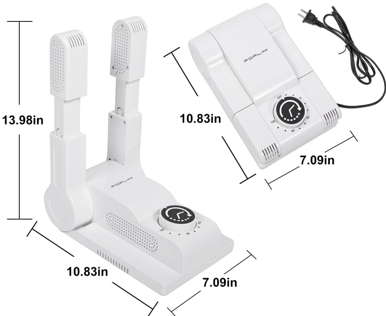
Image: The FORLIM Boot Dryer displayed with its key dimensions (length, width, height) indicated.
